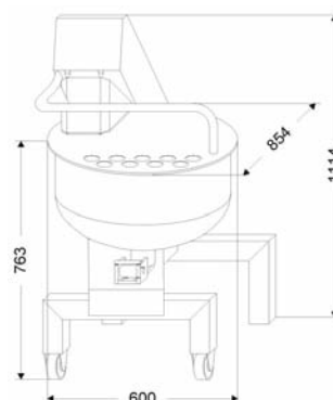
Dimensions PMX90 PMX90CM
